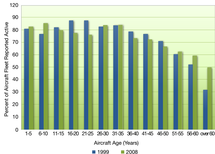
FIGURE 6.1 Change in Aircraft Utilization with Age – 1999 and 2008
