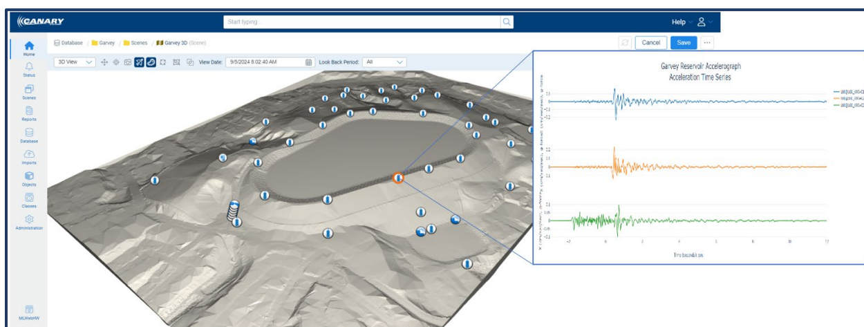
Figure 4-5: Garvey Reservoir Dam Monitoring System Dashboard and Recent Earthquake Data
